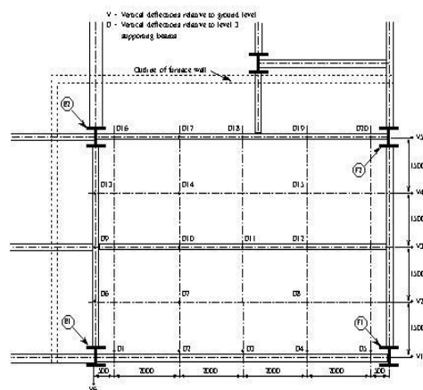
Test 3 - Transducer Positions for Measuring Vertical Deflections
