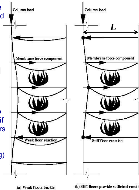
(a) Weak floors buckle
